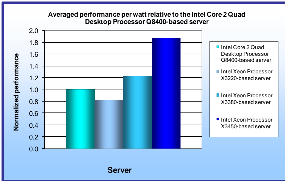
Figure 2: Normalized performance-per-watt results of the Intel processor-based servers across the three benchmarks relative to the Intel Core 2 Quad Desktop Processor Q8400-based server. Higher numbers are better.
