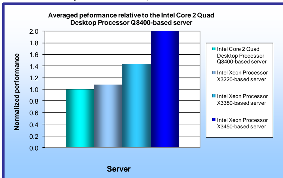
Figure 1: Performance of the Intel processor-based servers across the three benchmarks relative to the Intel Core 2 Quad Desktop Processor Q8400-based server. Higher numbers are better.
