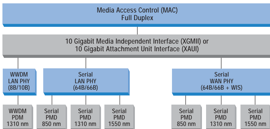
Figure 1. The architectural components of the 802.3ae* standard.
